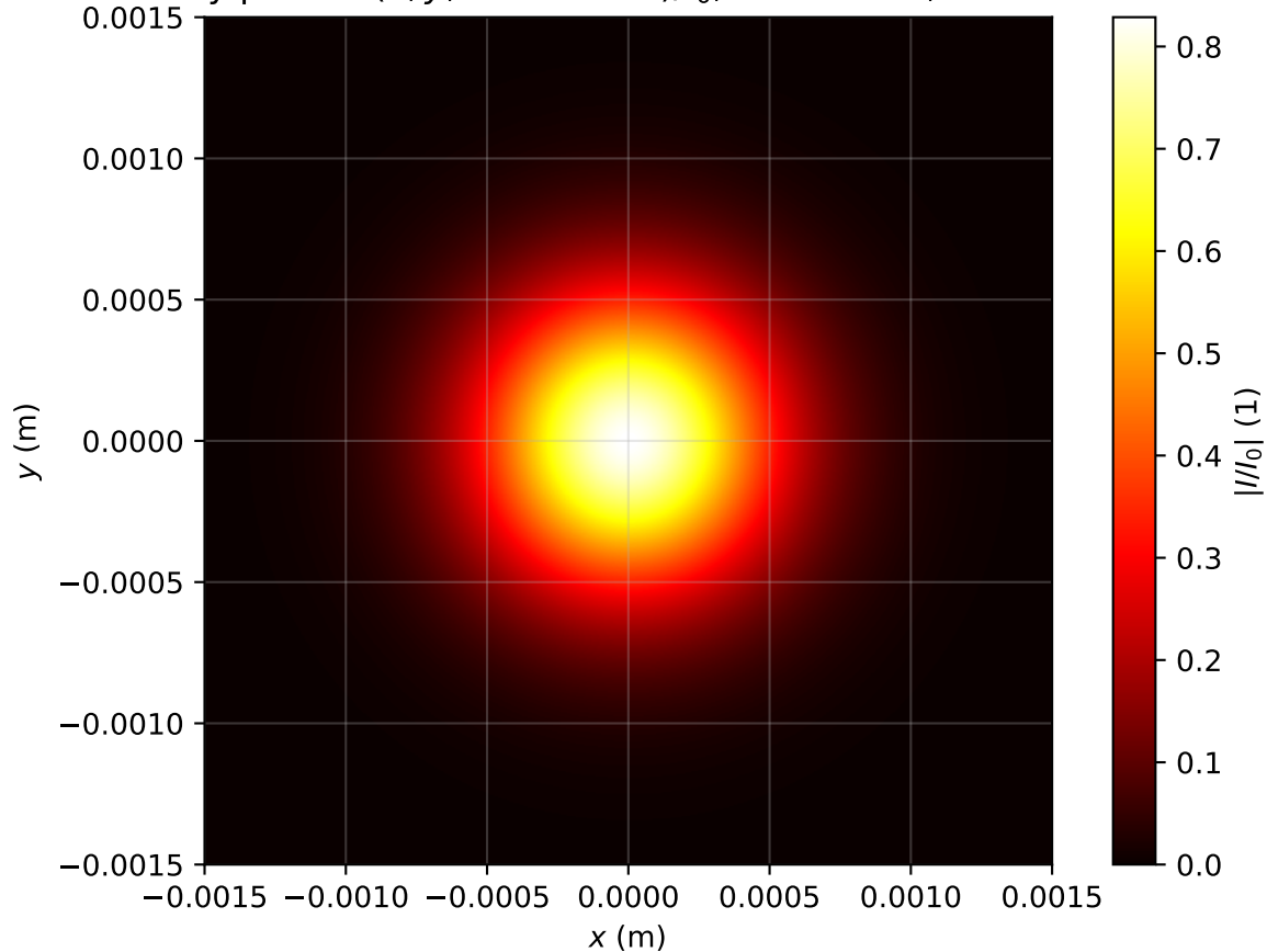
Intensity profile I(x, y, z = 1.194m)/I_0 , P_{in}=0.2P_{cr} , artificial time
